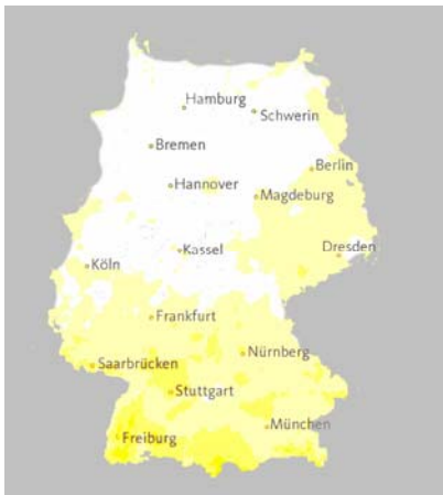
Figure 2: Germany Insolation
