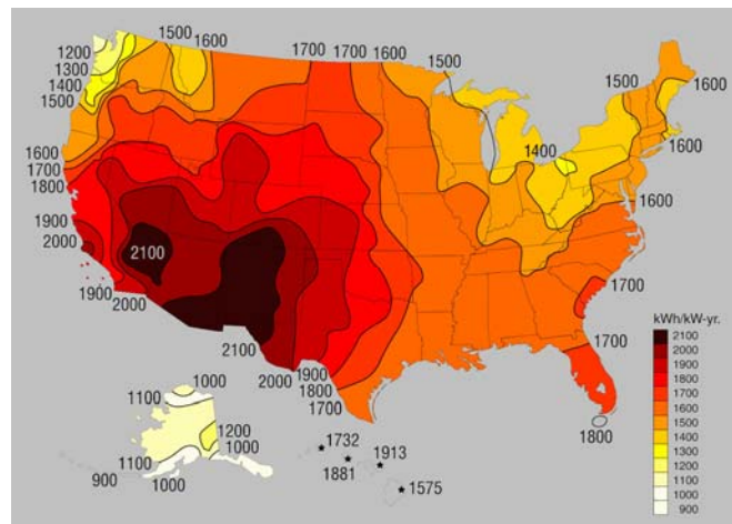
Figure 3: U.S. Insolation
