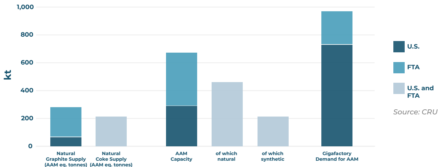
Figure 7: Graphite Raw Material Balance in U.S. and FTA, 2030
